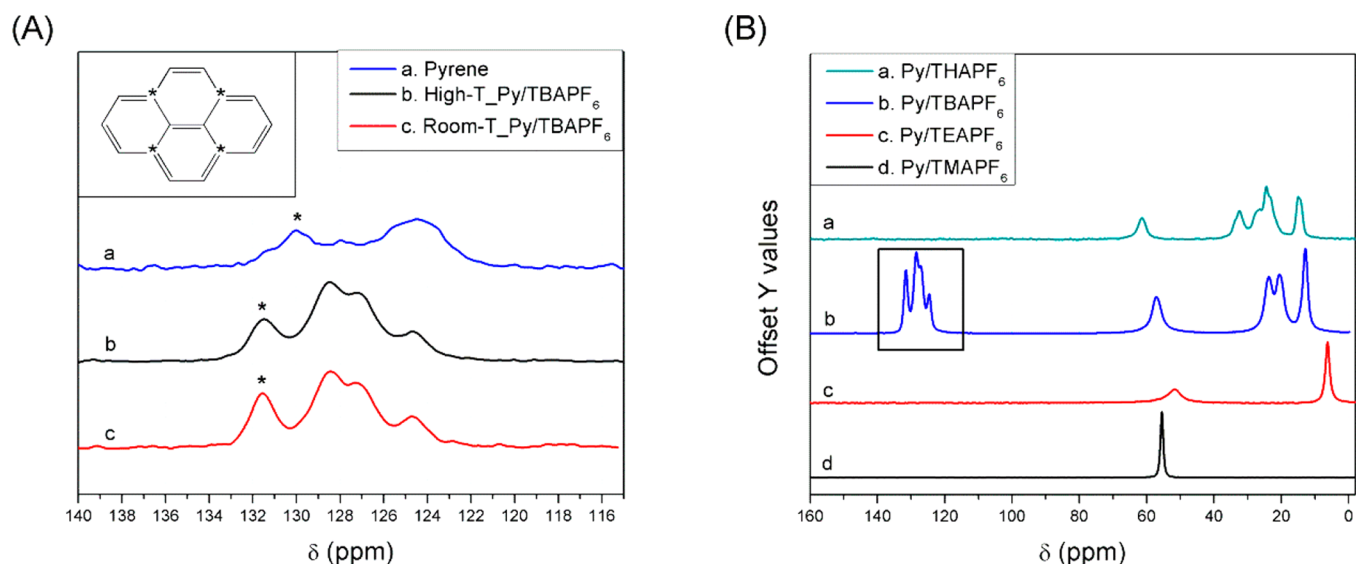
Figure 5. ^{13}\text{C} NMR spectra of (A) pure Py film (blue), Py/TBAPF 6 film prepared by high- T evaporation (black) and room- T evaporation (red), which is the blowup of the box in (B). The inset shows a pyrene molecule where the asterisks represent the carbons for the corresponding NMR shifts around 130–132 ppm. (B) Complete NMR spectra of Py/TMAPF 6 (black), Py/TEAPF 6 (red), Py/TBAPF 6 (blue), and Py/THAPF 6 (green) films prepared by room- T evaporation.
