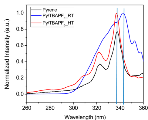
Figure 8. Fluorescence excitation spectra of Py (black), room- T prepared Py/TBAPF 6 film (blue), and high- T prepared Py/TBAPF 6 film (red), monitored at two emission wavelengths (A) 375 nm ( I_{mon} ) and (B) 455 nm ( I_{exc} ).
